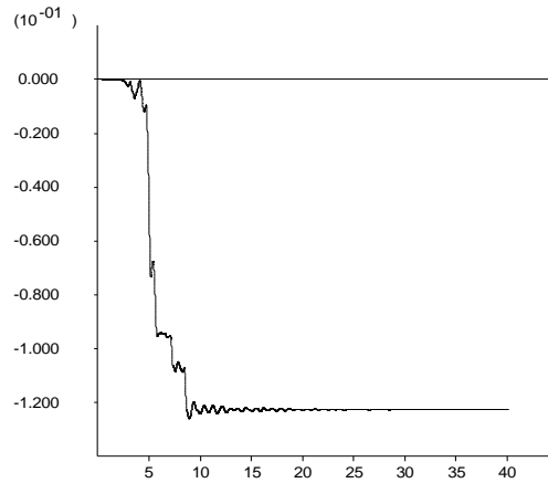
Fig.6. Vertical permanent displacement in crest after employing Loma Prieta earthquake record (Coralitos Station)
