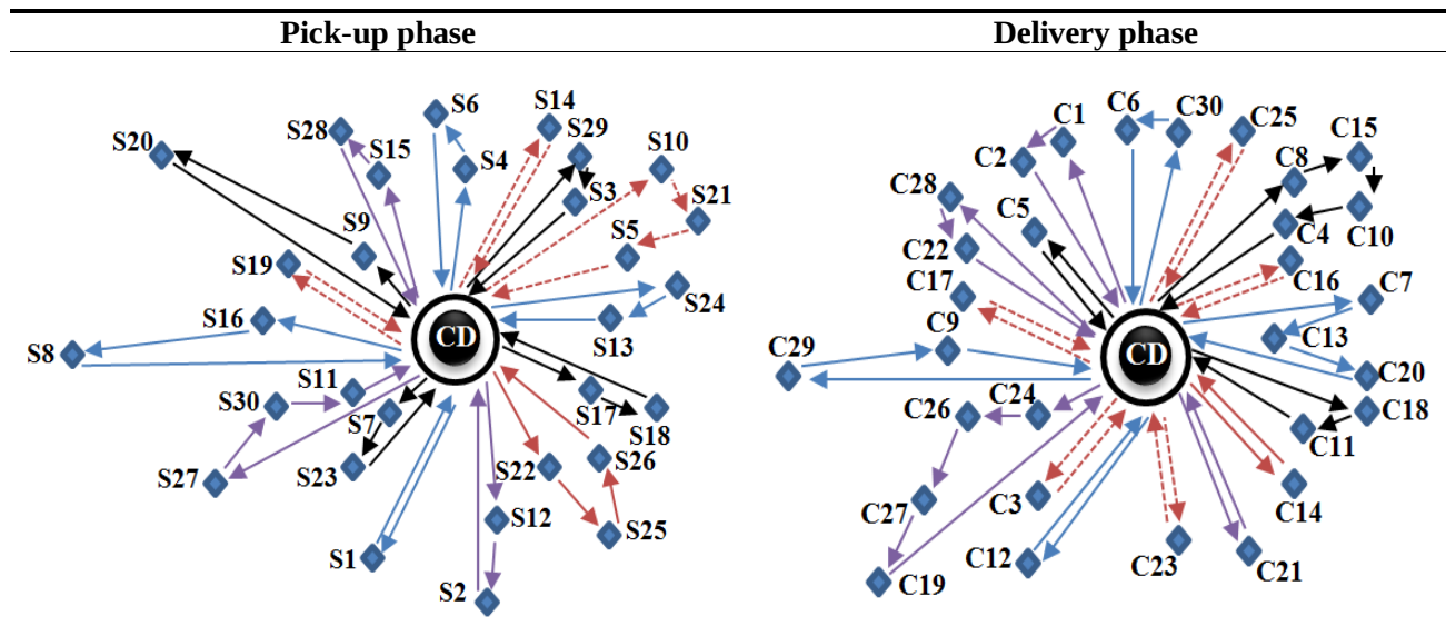
Figure 9. The best routing-cost solution to the instance 30 a using the MA algorithm.
